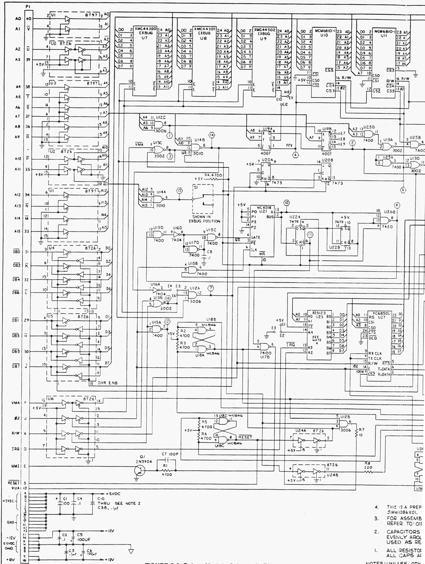
FIGURE 5-6. Debug Module Schematic Diagram
